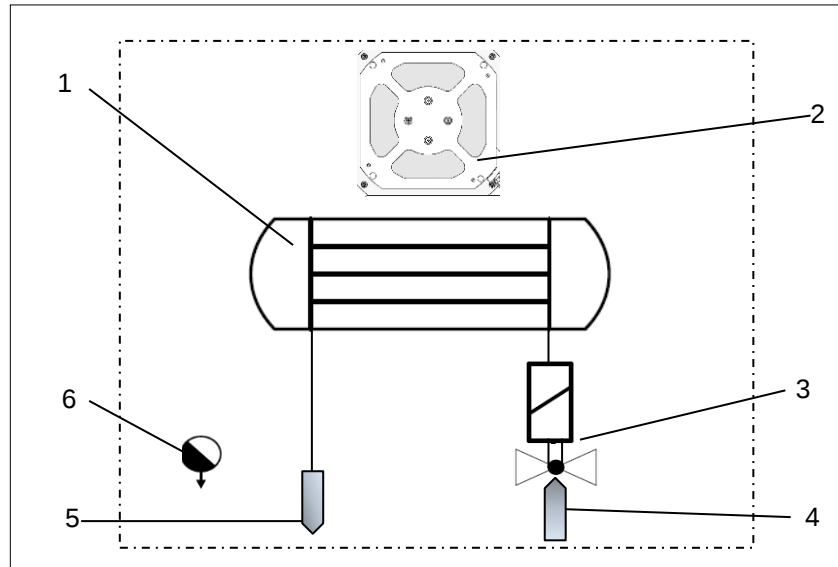
Figure 3 - Refrigerant circuit
