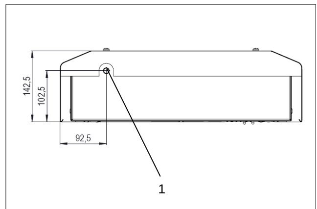
Figure 14 – Condensate drain connection PWS
