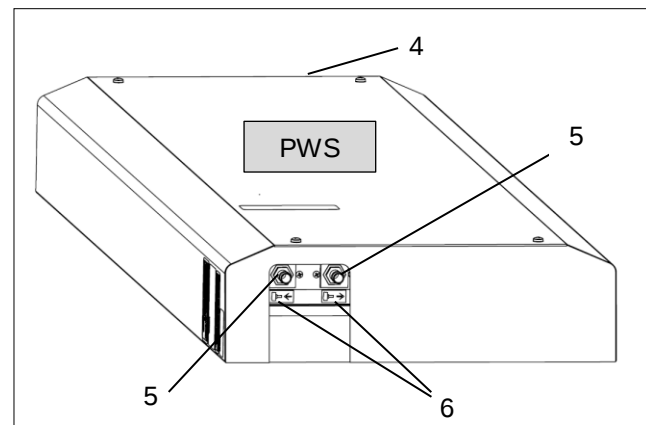
Figure 12 – Cooling water connections with threaded hose nozzles (top view)
