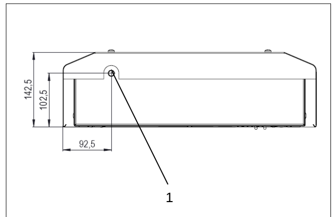
Illustration 14 – Raccordement de l'évacuation du condensat PWS
