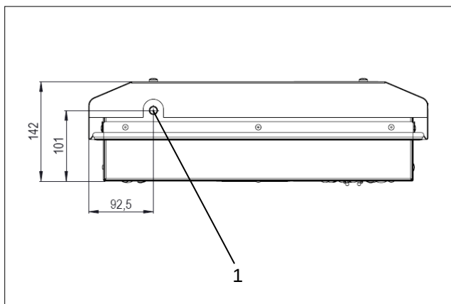
Figure 13 – Condensate drain connection PWI
