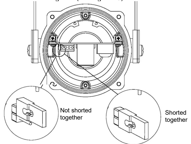
Fig. 6 Header Pin Settings
